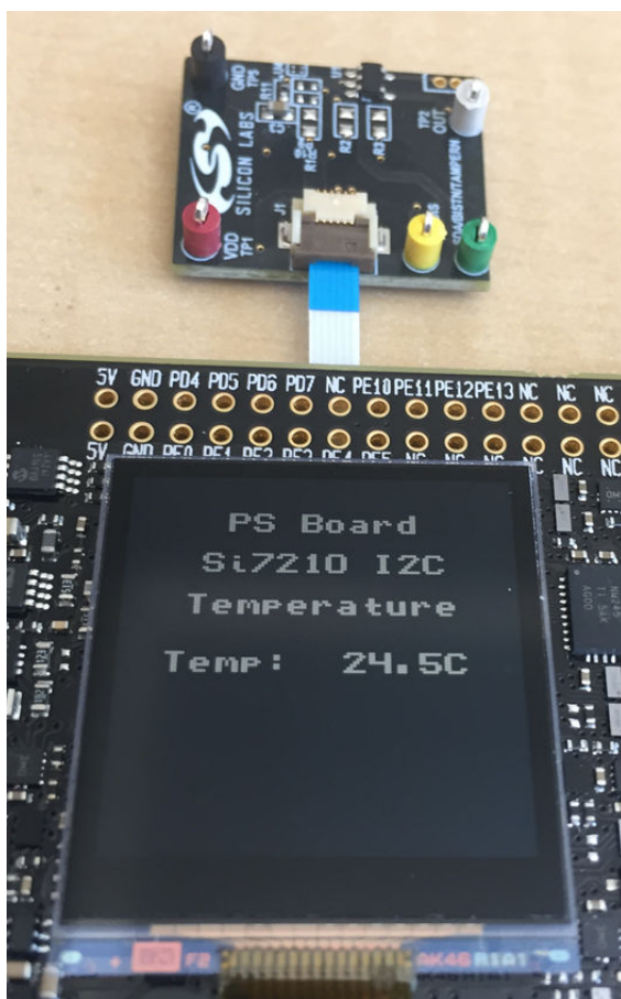
Figure 1.8. Temperature Sensor
